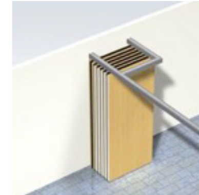
Double point suspension, panels have 2 multi directional rollers with 1 roller always on the centreline of top tracks
